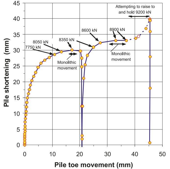
Fig. 14. Pile shortening versus pile toe movement in Shinho head-down test.
