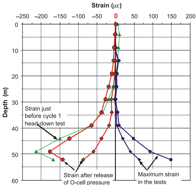
Fig. 9. Test-induced change of strain values measured at the maximum Shinho O-cell loads.
