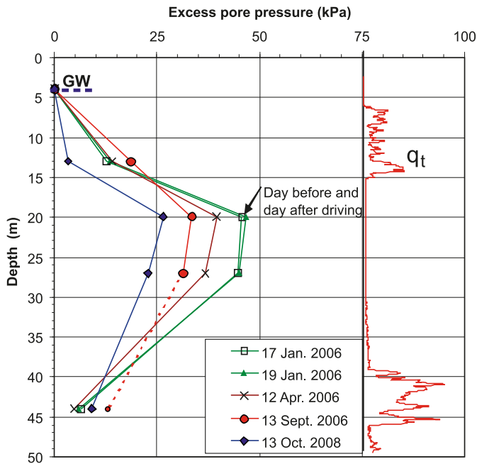
Fig. 2. Distribution of pore pressure measured about 10 m away from the Shinho O-cell test pile. GW, groundwater table.
