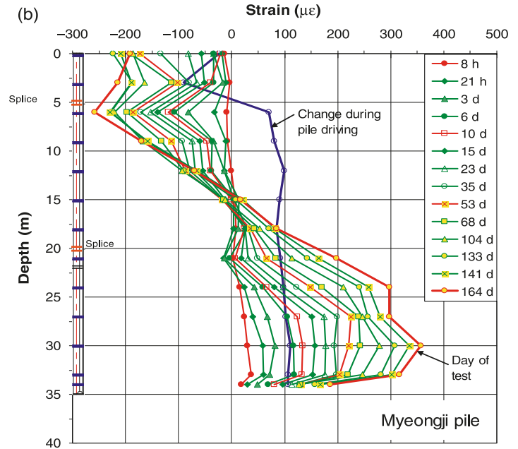
Fig. 6. Distribution of strain in (a) Shinho pile and (b) Myeongji pile at selected times after grouting until day of static loading test. d, days.
