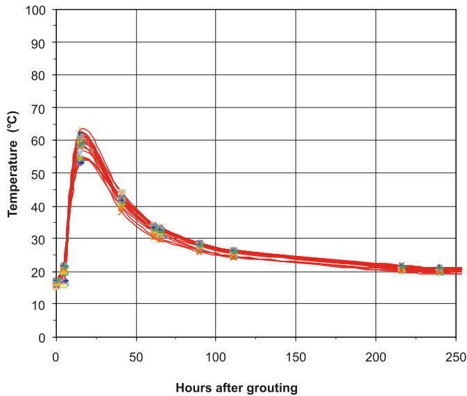
Fig. 3. Temperatures measured at the gage levels in the Shinho test pile during the first 250 h after grouting the pile.
