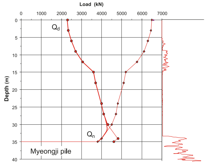
Fig. 20. Long-term resistance and load distributions for a construction pile similar to the test pile at the Myeongji site.
