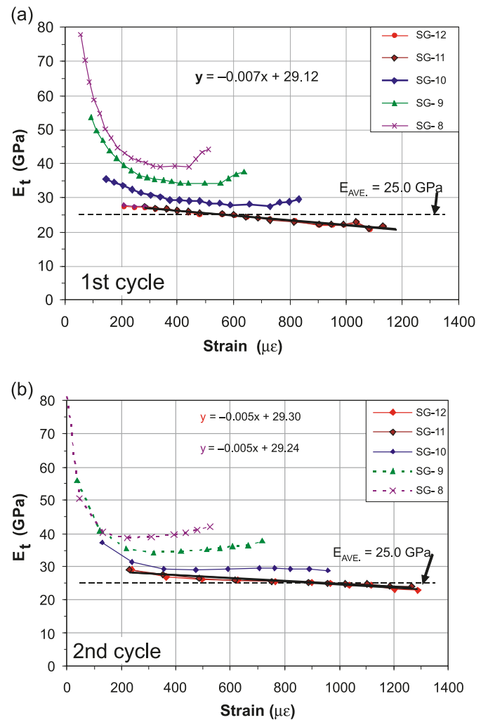
Fig. 12. Tangent modulus graph from measurements of load, E_t , and strain in the Shinho pile: (a) stage 2, cycle 1 and (b) stage 2, cycle 2 (y and x are variables in the linear regression equation).
