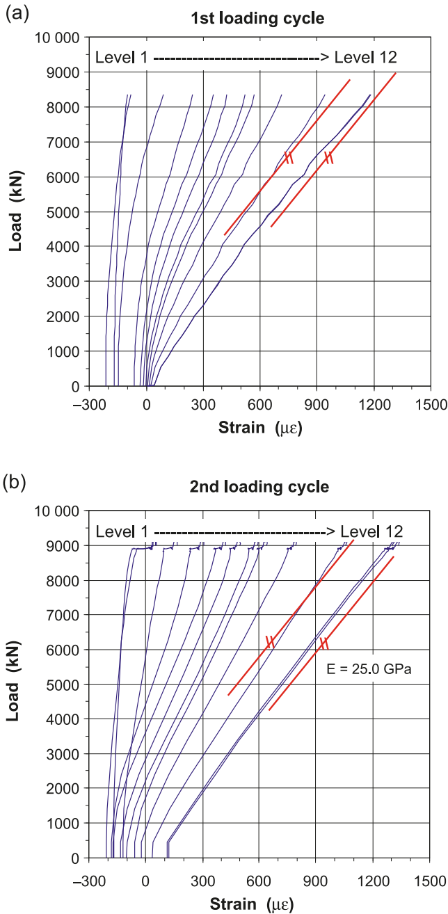
Fig. 11. Load–strain recorded in Shinho (a) cycle 1 and (b) cycle 2 strain gages.
