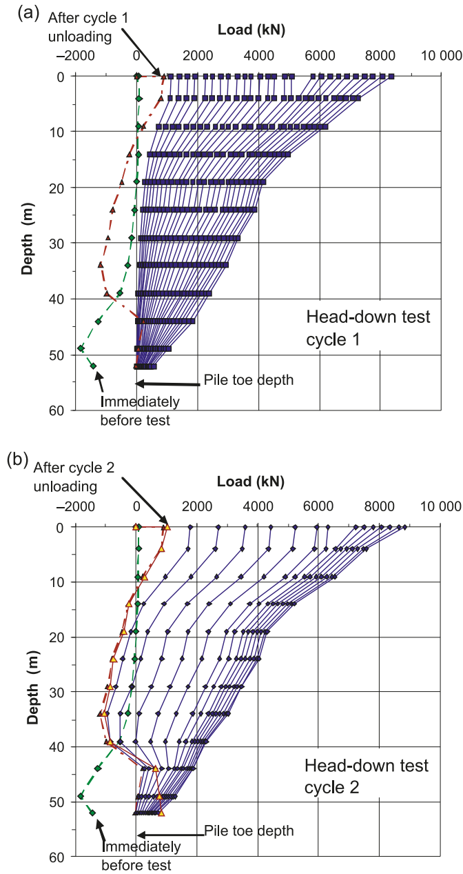
Fig. 13. Distribution of load in Shinho (a) stage 2, cycle 1 and (b) stage 2, cycle 2 from the imposed strains uncorrected for residual load. Also shown are the load distributions after unloading the pile after the O-cell test cycle 2 and after the head-down test (a) cycle 1 and (b) cycles 1 and 2.
