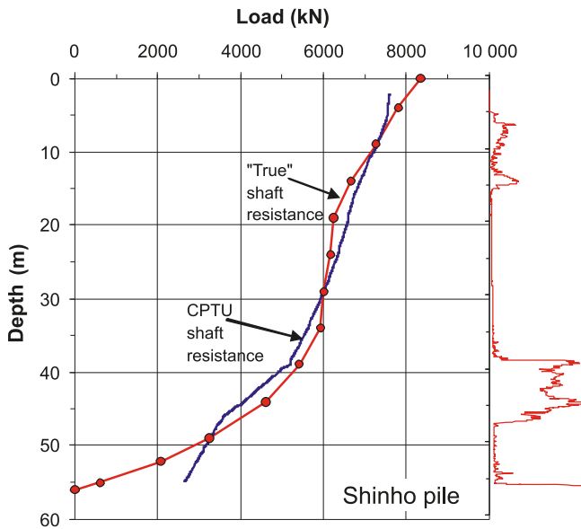
Fig. 17. “True” resistance distribution (curve F in Fig. 16) in the Shinho pile test and shaft resistance calculated from the CPTU method. The latter is offset to provide a better comparison to the “true” distribution.
