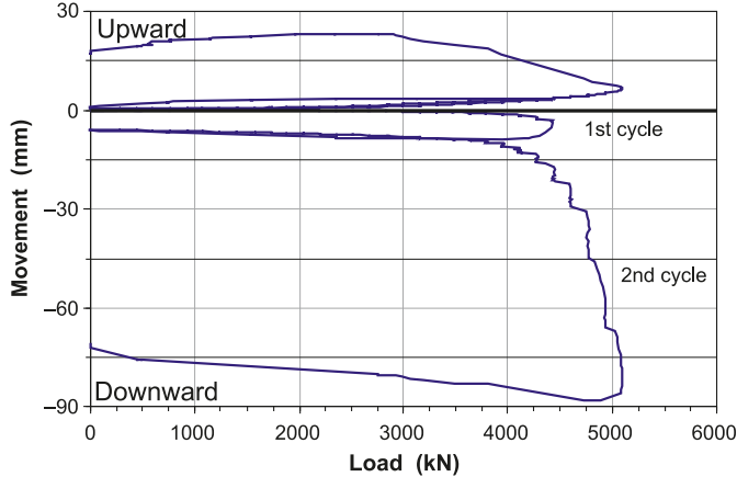
Fig. 7. Upward and downward movements of the Shinho O-cell plates.
