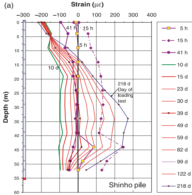
Fig. 6. Distribution of strain in (a) Shinho pile and (b) Myeongji pile at selected times after grouting until day of static loading test. d, days.
