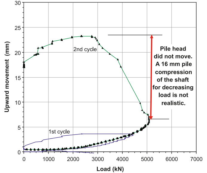
Fig. 8. Upward movements of the Shinho O-cell plates plotted to enlarged scale.
