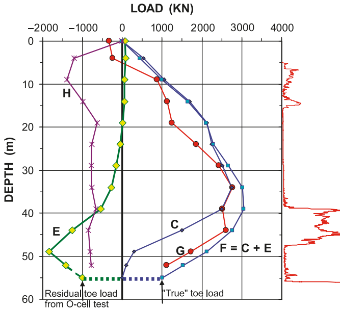
Fig. 16. Residual load (C) in the Shinho pile determined by the method proposed by Fellenius (2004, 2009) for stage 2 test and residual load (F) for stage 1 test after adding in the release of load subsequent to unloading the stage 1 test (O-cell test).
