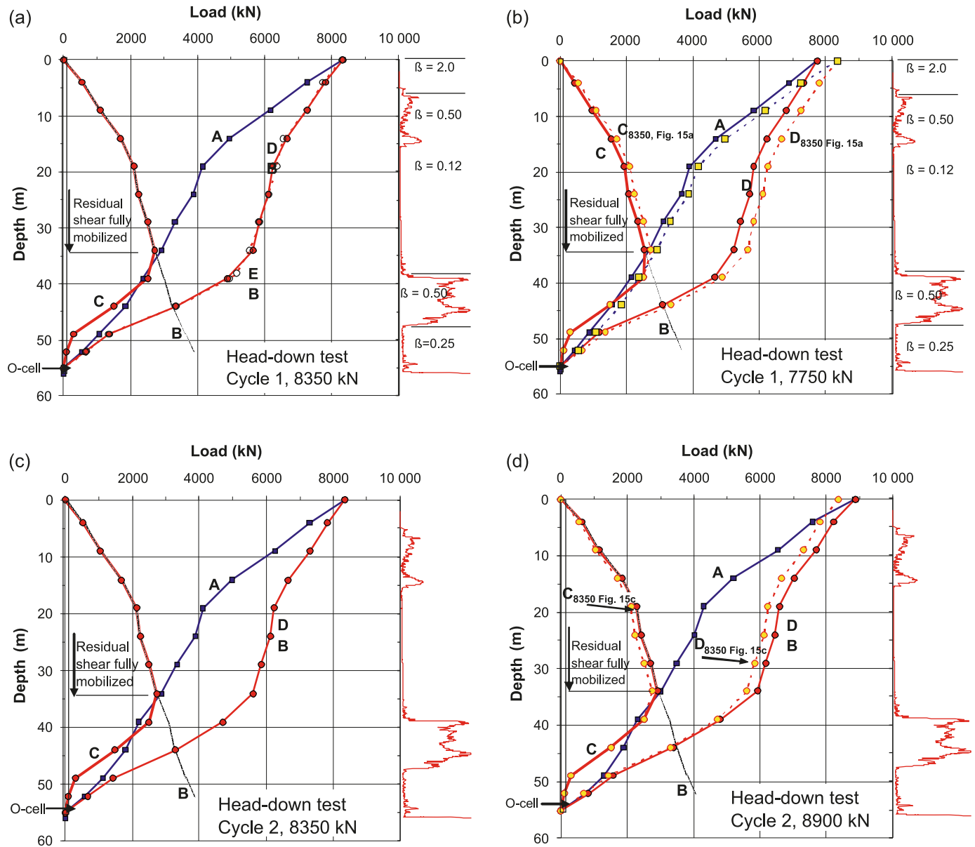
Fig. 15. Construction of the Shinho residual load: (a) cycle 1 for 8350 kN applied load; (b) cycle 1 for 7750 kN applied load; (c) cycle 2 for 8350 kN applied load; (d) cycle 2 for 8900 kN applied load.
