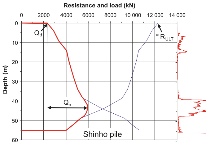
Fig. 19. Long-term resistance and load distributions for a construction pile at the Shinho site, which is similar to the test pile at the Shinho site. Q_n , drag load; R_{ULT} , ultimate resistance.
