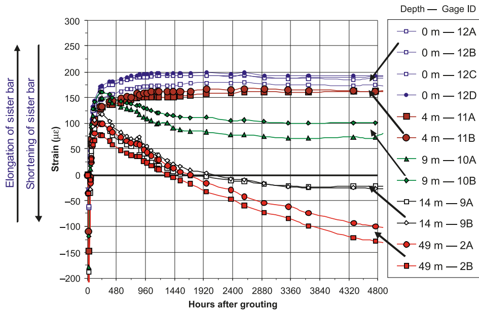
Fig. 5. Strains measured in the Shinho test pile during 200 days after grouting the pile.
