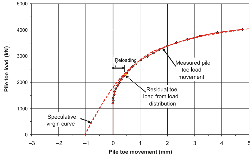
Fig. 21. Myeongji pile: toe resistance evaluated from the strain gages versus measured pile toe movement.
