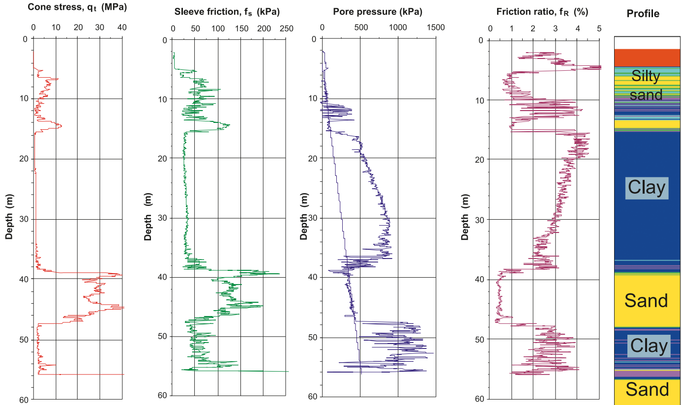
Fig. 1. CPTU at Shinho: q_t , cone stress; f_s , sleeve friction; U_2 and u_0 , pore pressure; f_R , friction ratio.
