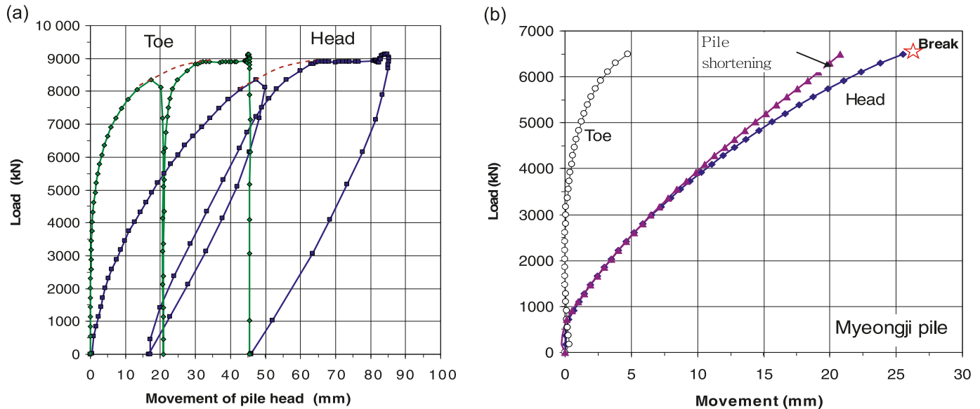
Fig. 10. Pile head and pile toe load–movements measured in the (a) Shinho and (b) Myeongji head-down tests.
