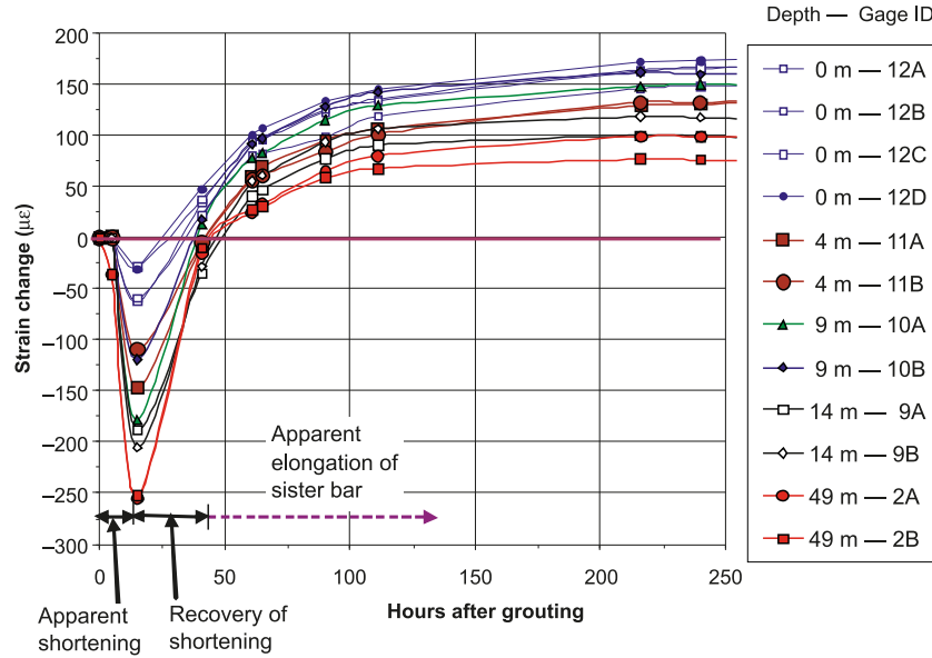
Fig. 4. Strain change measured at select gages in the Shinho test pile during the first 250 h after grouting the pile.
